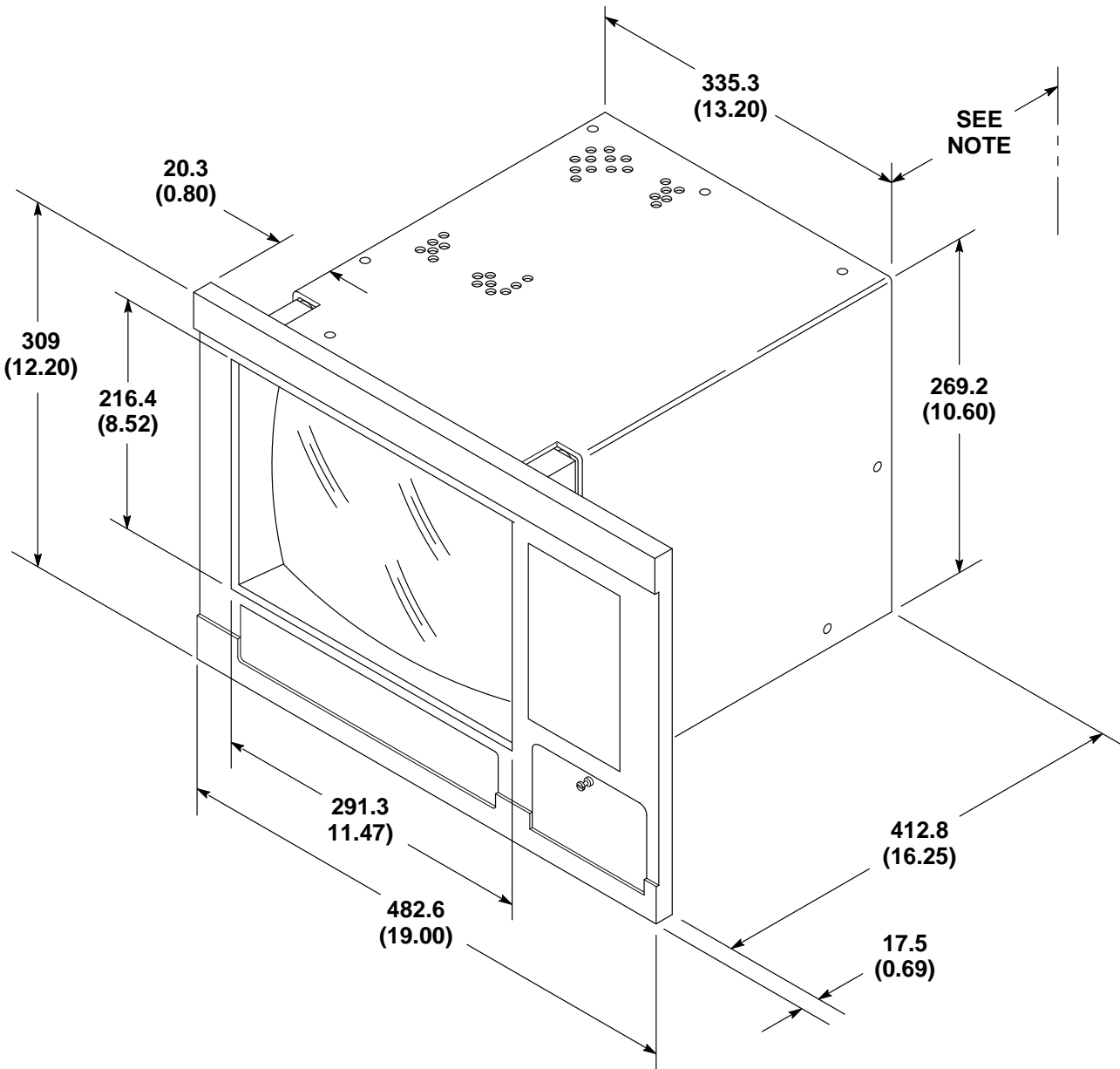
Figure 2 Bulletin 6156 Industrial Monitor (Without Keypads) Physical Dimensions
