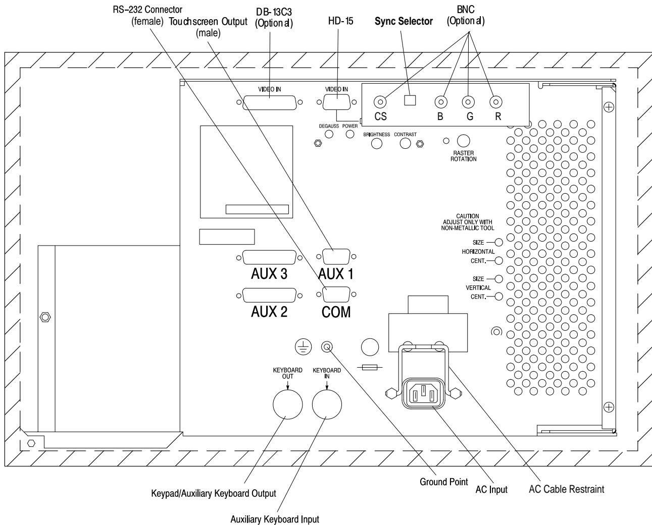
Figure 7 Rear Panel of Monitor
