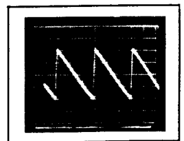
⑩ 5V/DIV, 5ms/DIV
